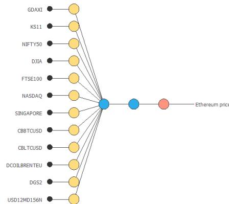
Fig. 14. Final architecture
