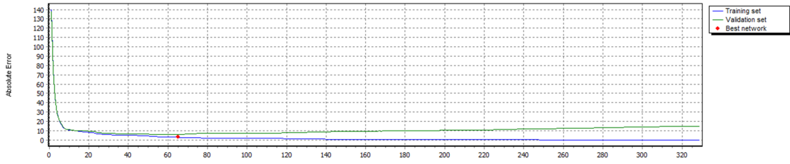
Fig. I. Training graph
