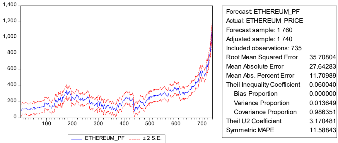
Fig. V. ETH-price forecasting
