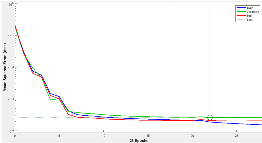
Fig. 10. Network Performance
