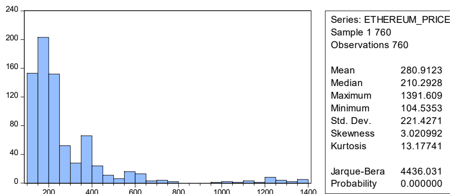
Fig 15. Ethereum price histogram
