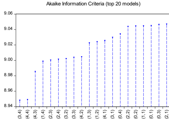
Fig. 16. Akaike information criteria (top 20 models)
