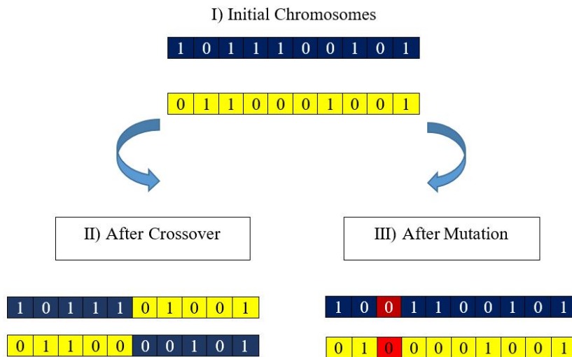
Fig. 3. Genetic algorithm process
